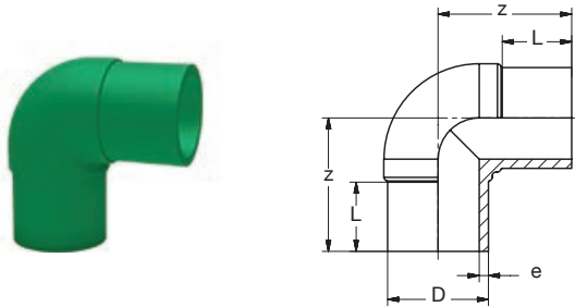
BR PP-RCT Winkel 90° lang st SDR7,4 grün BR PP-RCT Elbow 90° long butt SDR7.4 green
