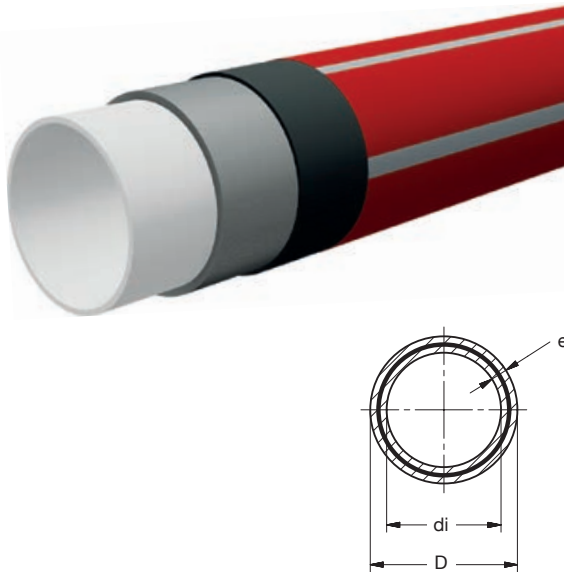
BR CFR Pressure pipe FIRETEC 1.6MPa red
