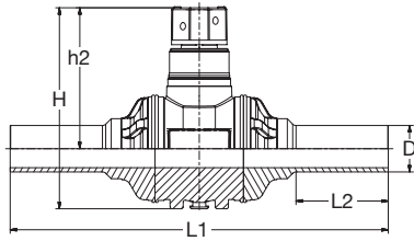
BR PE100 Kugelhahn Abwasser PN10 lang Anschlüsse SDR11 schwarz BR PE100 Ball valve sewage water PN10 long connectors SDR11 black
