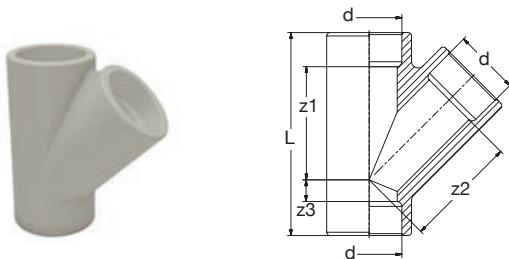
BR PP-INDUSTRIAL Abzweig 45° 20°C/1,0MPa grau BR PP-INDUSTRIAL Branch 45° 20°C/1.0MPa grey
