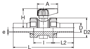
BR PE100-PVC-U Kugelhahn lang Anschlüsse SDR11 schwarz BR PE100-PVC-U Ball valve long connectors SDR11 black
