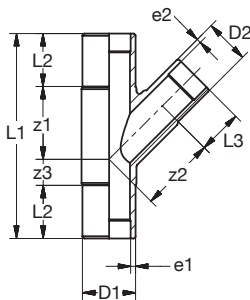
BR PE100 Abzweig 45° red lang SDR17(-11) schwarz BR PE100 Branch 45° red long SDR17(-11) black
