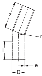
BR PE100 Rohrbogen 22° nahtlos lang SDR11 schwarz BR PE100 Pipe bend 22° seamless long SDR11 black
