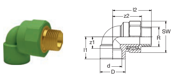
BR PP-R-RG Ü-Winkel 90° AG-keg grün
